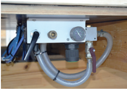
Includes pneumatics systems for the central air supply and controlling the C-PowerTec clamping beams
