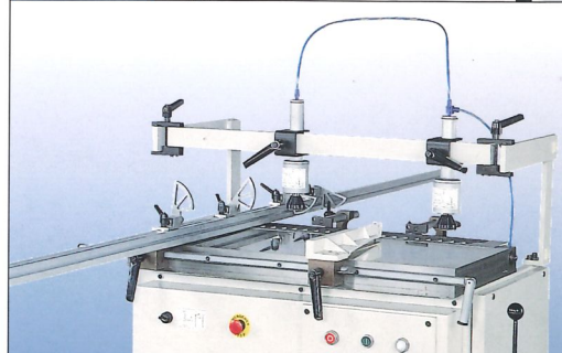
Optional: Long auxiliary aluminum fence(3M) & stoppers.
