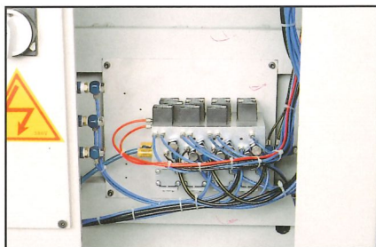
Pneumatic sequence controller: All pneumatic compounds are directly installed onto the integrated circuit distributor. Very easy change pneumatic parts.(Optional)
