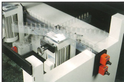
Pictures illustrates vertical boring units of LB-55/63 can be rotated for PARALLEL & TANDEM operation.
