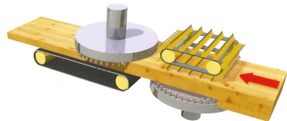
Double-side calibrating milling machines Working width from 200 up to 1350 mm
