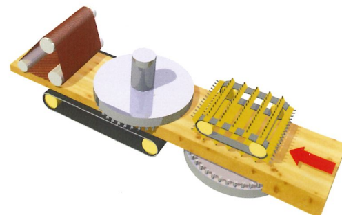
Double-side calibrating milling machines with sanding aggregate Working width from 400 up to 1350 mm
