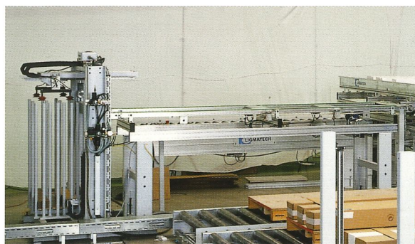
Magazine for cardboard strips
