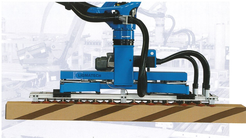
Universal vacuum picker arm
