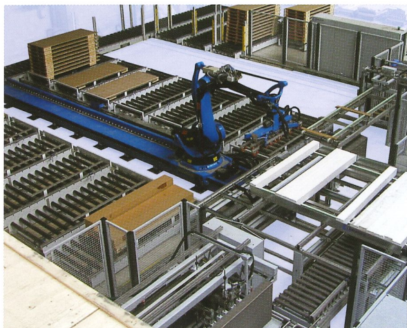
Palletizing by commission
