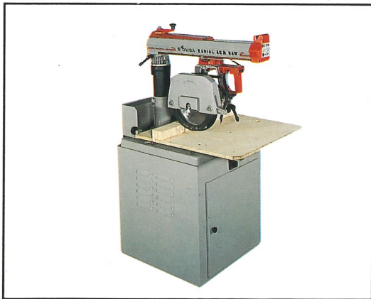
Cod. 720126000 RN 350 Cod. 7201060100 RN 450 BASAMENTO ASPIRANTE DUST EXTRACTION UNIT ABSAUGSCHRANK BATH ASPIRANT AFZUIGINRICHTIG SOPORTE ASPIRANTE
