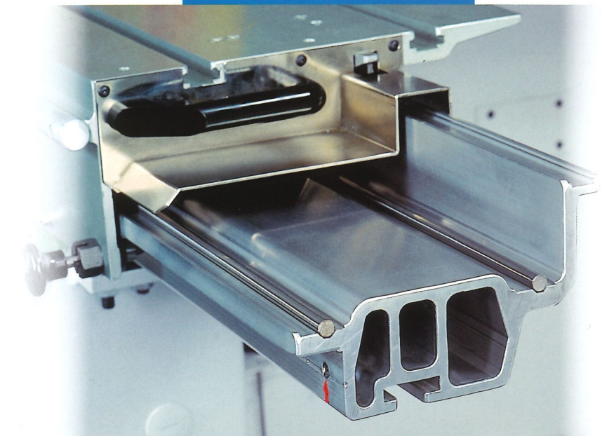
Double sliding table with hardened and ground guiding rails. Standard.
