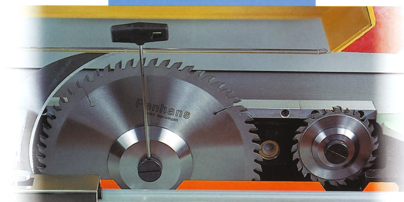
Quick blade clamping system APA. Standard.
