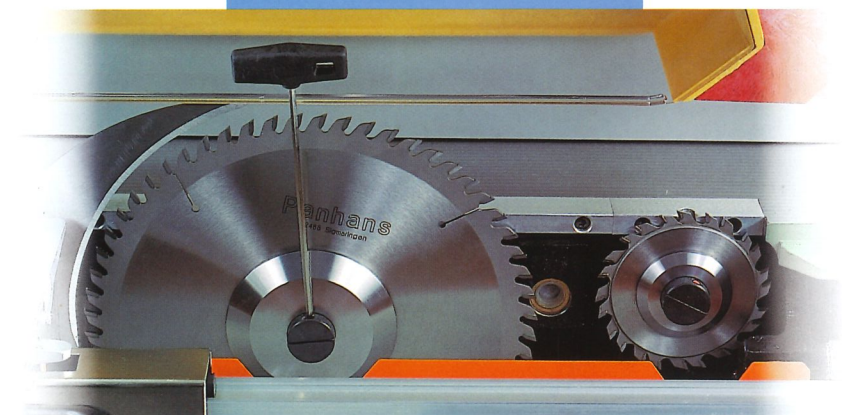
Quick blade clamping system APA. Standard.
