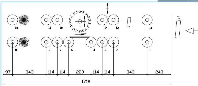
Fig. 26 Schematic view of K34G-O with special anti-kickback device
