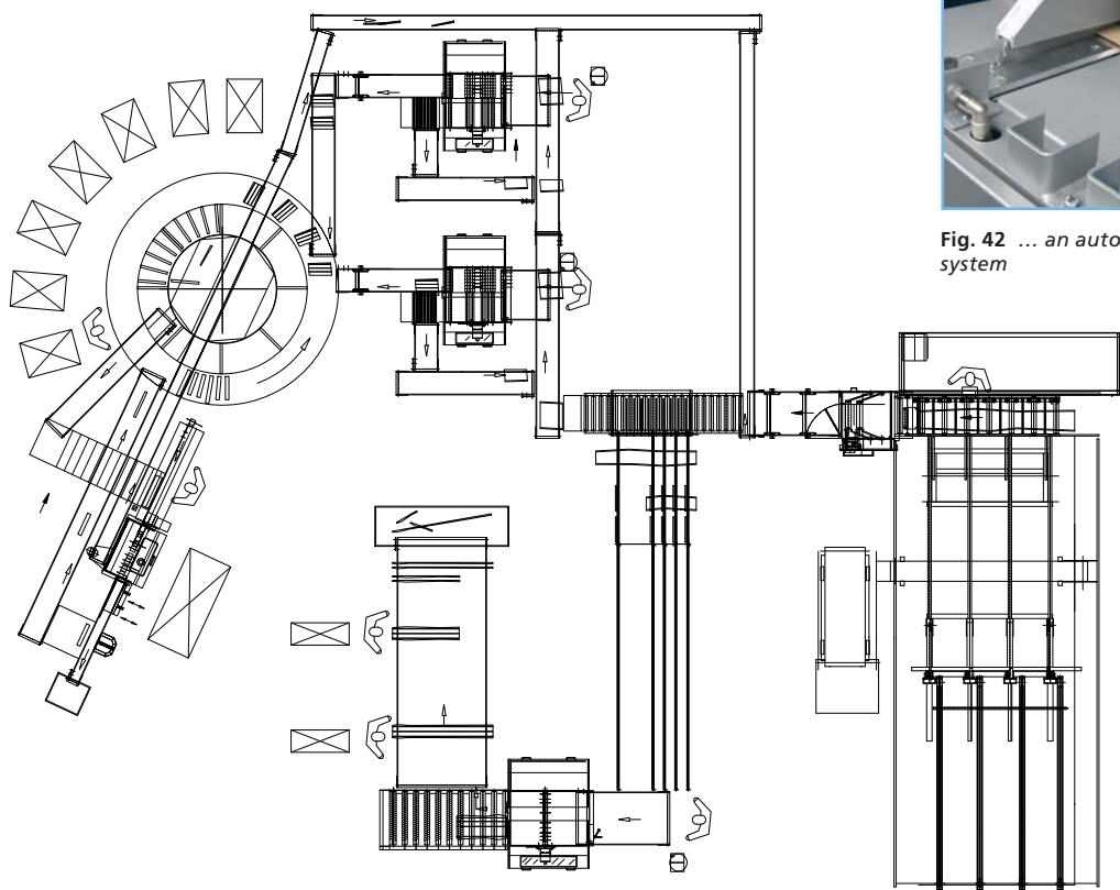
Fig. 43 Rip and cross-cut system for solid parquetry (battens, flooring planks) incl. pre-cross-cutting, ripping, cutting to final length and sorting carousel
