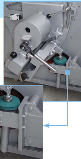
Fig. 12 Height adjustment of saw shaft by an electrically driven lifting spindle
