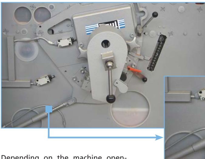
Fig. 13 Height adjustment of saw shaft by a hydraulic cylinder
