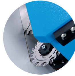
Scoring unit with 2 split saw blades Incisor de doble sierra
