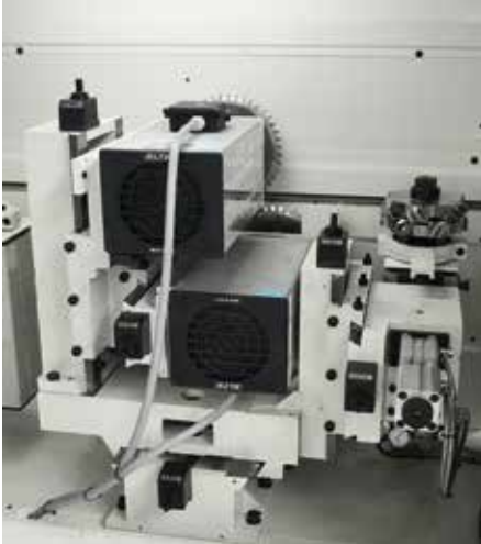
Anti-chipping and double hogging unit. Ideal for high levels of chipping.
