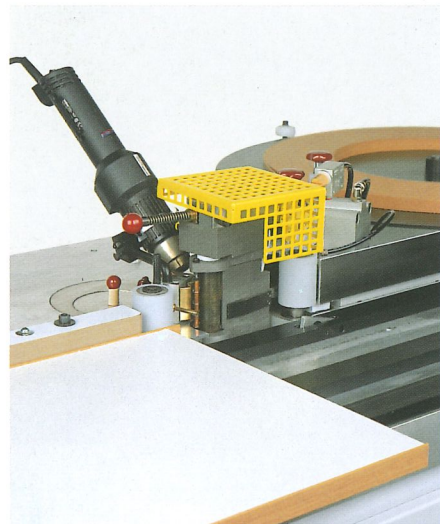
Processing of straight edges. Hot air unit for thick PVC edges (option).
