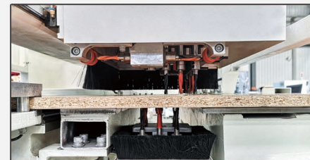
6-sided drilling completed in one cycle
