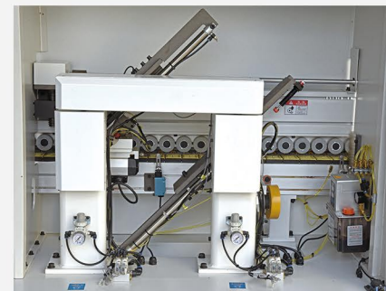
Two motors traveling on linear guides for end-trimming
