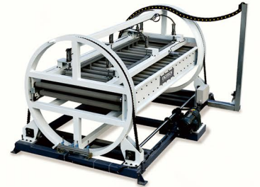
Barrel Turner
