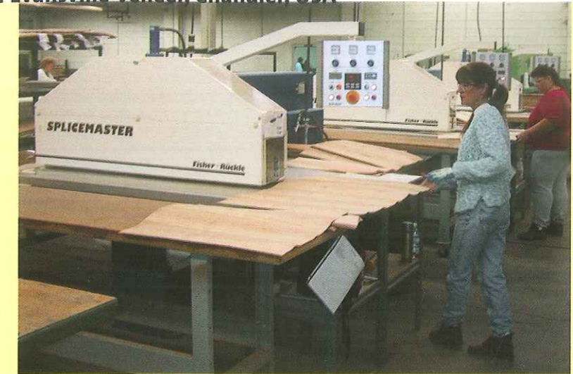
Splicemaster at hobb holzveredelung gmbh & co kg (hülsta-Group) Bad Bentheim, Germany
