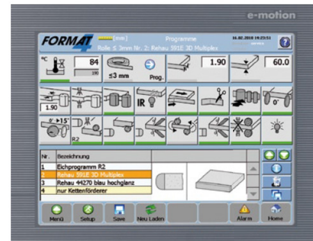
Radius trimming
