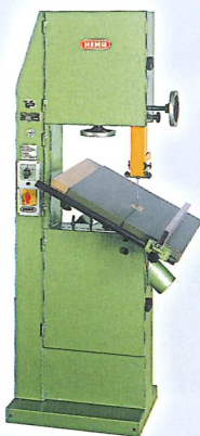
SR 400
