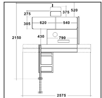
LAB 260 F Abmessungen in mm
