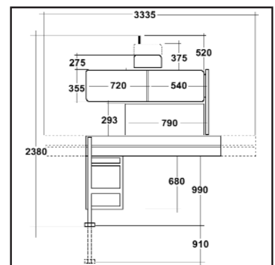
LAB 300 F Abmessungen in mm
