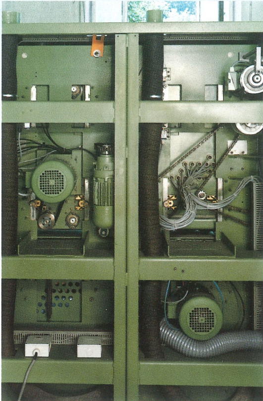
Abb./III. 2 Drives/Antriebe/Commandes
