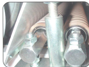
• Pressure roller with screw groove 壓料輪
