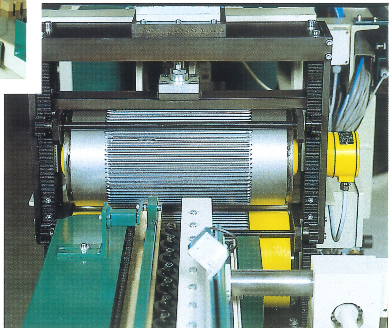
Acceleration Unit
