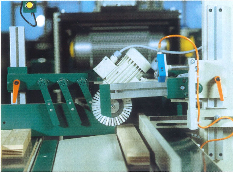
Transfer Unit
