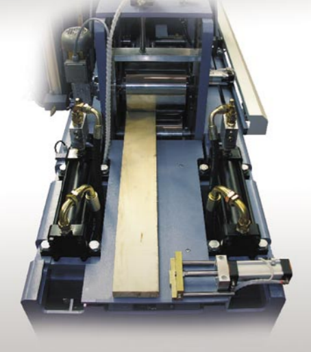
pressing cylinders
