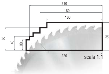
TR350 - Hp 4
