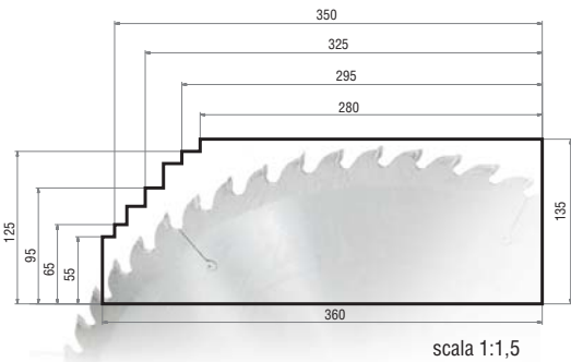
TR500 - Hp 10
