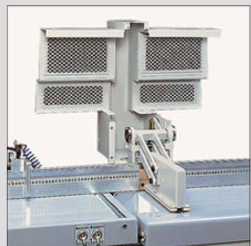
Pneumatic workpiece clamping
