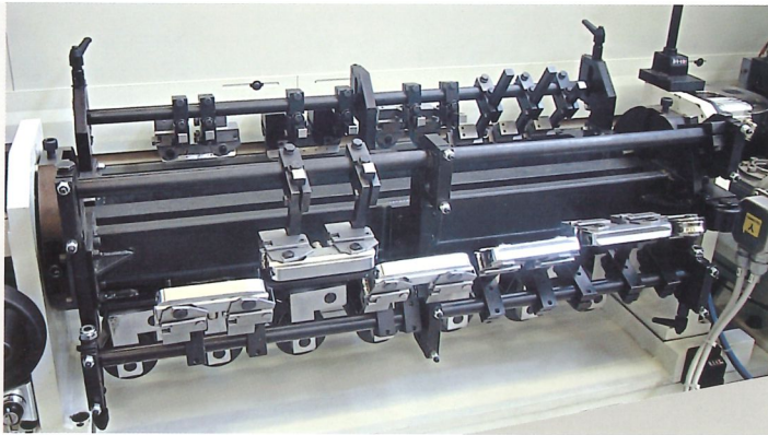
Cambio settori di pressione a revolver Pressure sectors change over by revolver system Cambio sectores de presión a revolver
