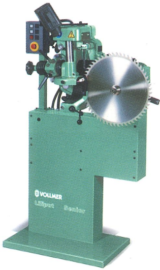
Liliput Senior Version for circular saw blades.
