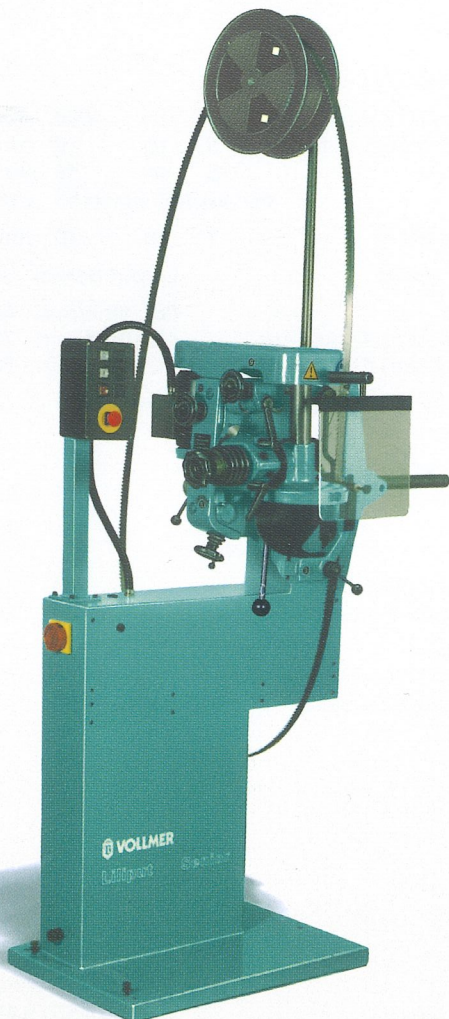
Liliput Senior Version for band saw blades.
