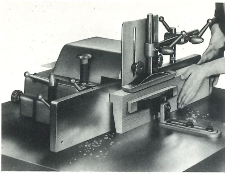
Deep Rail Moulding
