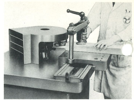
*Tenoning
