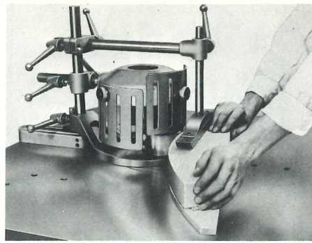
*Moulding Curved Surfaces
