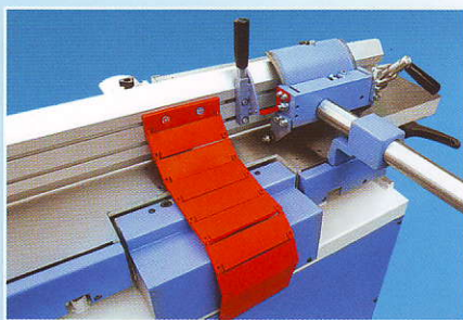
Професионален линеал (DMA 41) Profi Abrichtanschlag (DMA 41) Professional fence (DMA 41)
