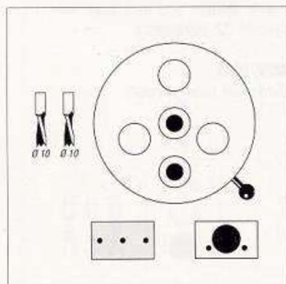
drill head position for press-in plate installation
