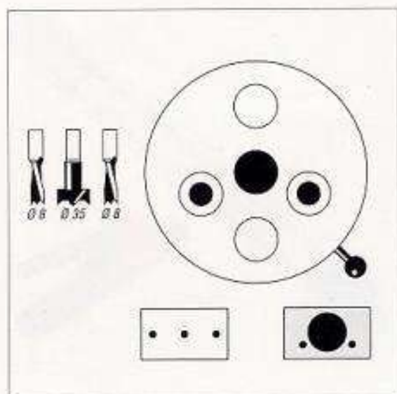
drill head position for hinge installation
