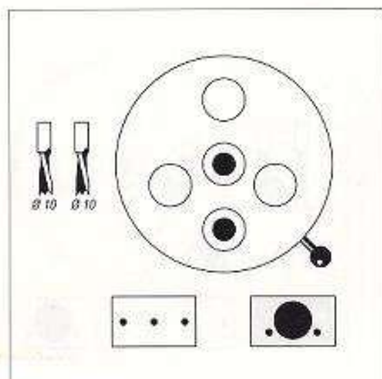
drill head position for front-fixing brackets
