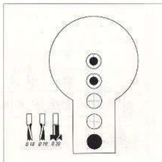
Drill bit arrangement for line-boring with the MZK.5000 BORING HEAD
