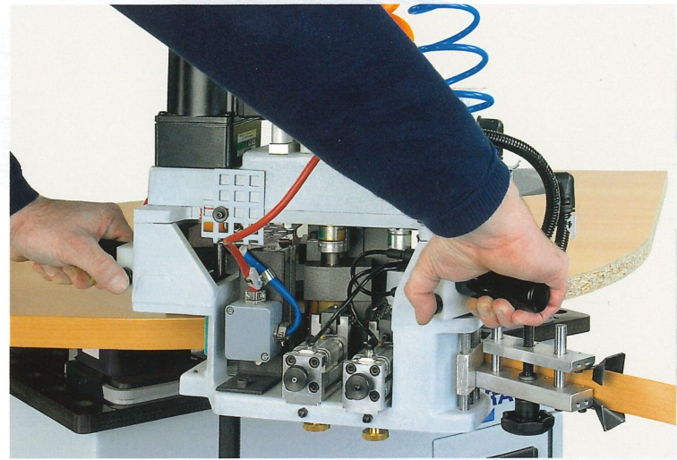
Freely moving gluing unit
