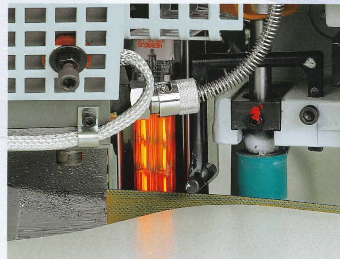
Infrared heating for thick PVC edgings
