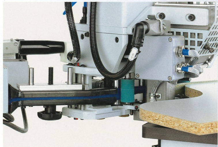
Safe edge material feed in case of stationary and manual operation
