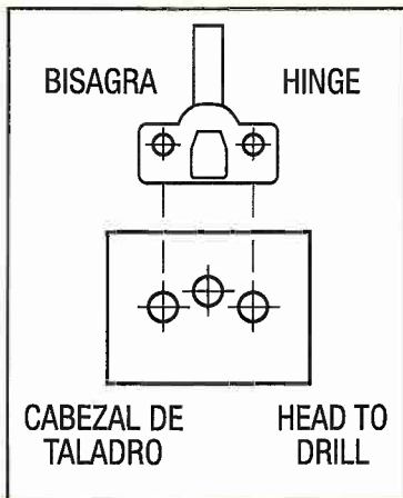
HEAD WITH 3 DRILLBIT-HOLDERS
