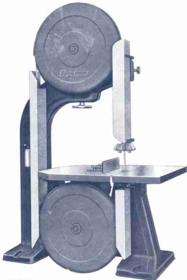
Art. 2220 Band saw - Mod. "ST 900" - "ST 1000" base in pressed steel - double frame - wheel in cast iron to rays.
