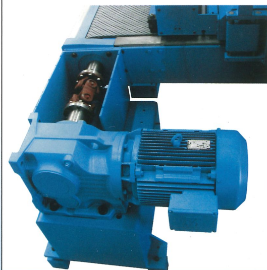
View of the heavy-duty drive unit linked with a cardan joint to the traction roller of the feed belt in a top calibrating machine
