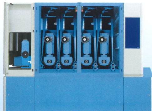
BA-R4 - grain highlighting machines with 4 steel brush units GS-25
