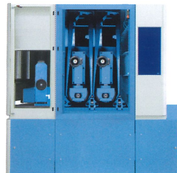
BA-R2 - grain highlighting machines with 2 steel brush units GS-25
