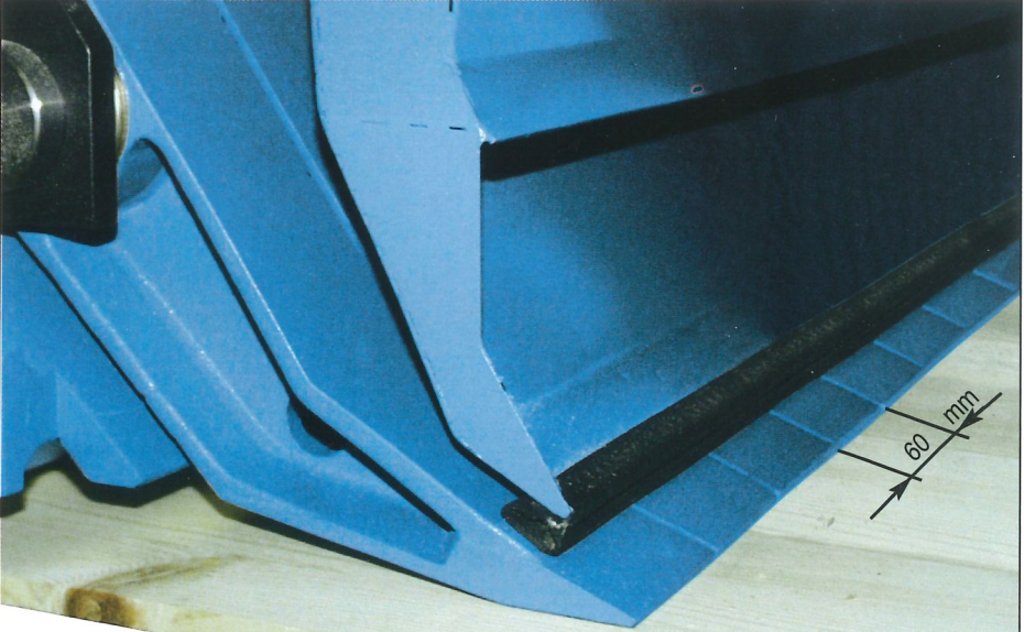
Infeed sectioned pressure unit + dust hood intake
