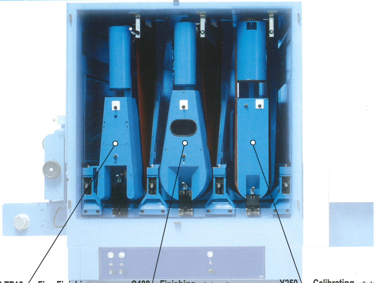
TP32 TP16 - Fine Finishing electronic controlled sectioned pad unit
