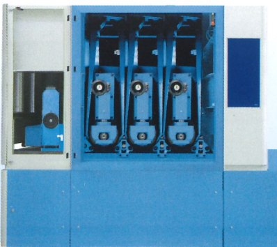
BA-R3 - grain highlighting machines with 3 steel brush units GS-25
