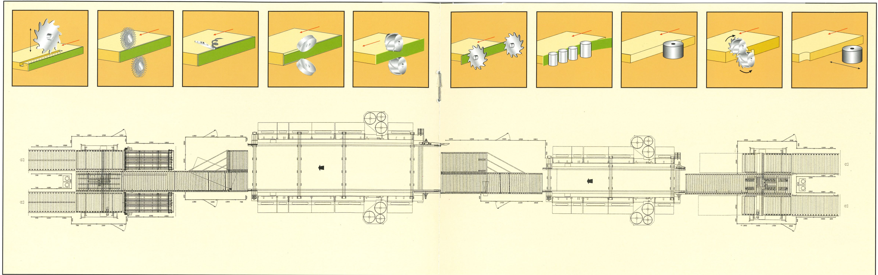
2) Gruppo incollaggio softforming Unit for softform glueing Grupo de encolado softforming Aggregat zum Softform- Anleimen Groupe encollage softforming
