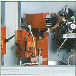
Toupie fissa porta-lama Fixed sawing unit Tupi fija porta-sierra Fixes Sägeaggregat Toupie fixe porte-lame
