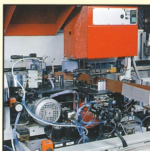
Gruppo incollaggio softforming Unit for softform glueing Grupo de encolado softforming Aggregat zum Softform- Anleimen Groupe encollage softforming
