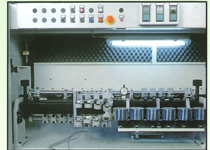
Gruppo incollaggio softforming Unit for softform glueing Grupo encolado softforming Aggregat zum Softform- Anleimen Groupe encollage softforming
