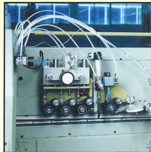
Inseritore IS Inserting units IS for edge T-slot insert Insertador IS Dichtungseinsetz-Aggregat IS Groupe d'introduction IS
