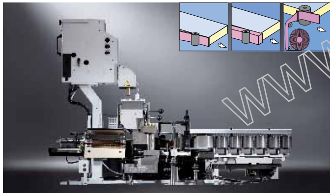
Hot-melt gluing unit A6
