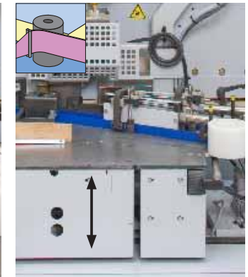
Magazine height adjustment
