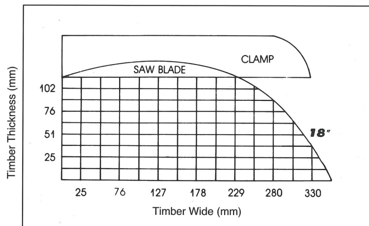
HCS-18 CAPACITY CHART
