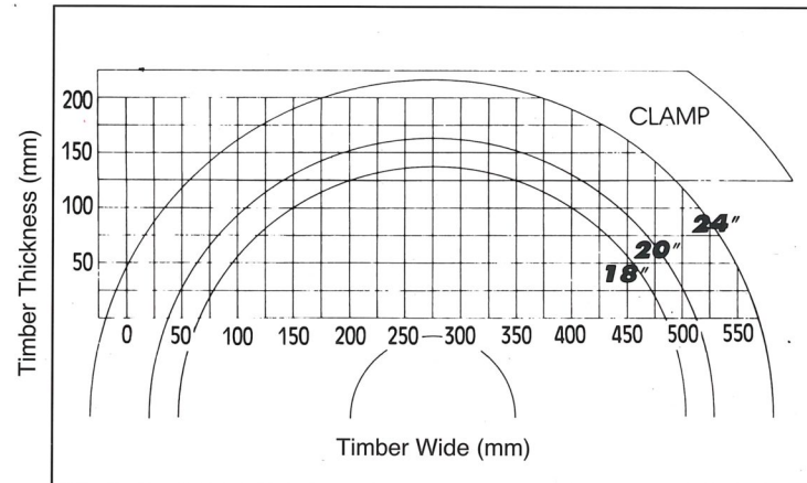
HCS-24 CAPACITY CHART
