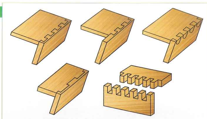
Examples of Joints
