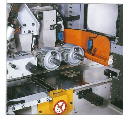
UPPER AND LOWER INFEED WITH PNEUMATIC CONTROL Rollers are powered, providing pneumatic control and a pressure gauge for a smooth feeding effect. A limit switch provides protection from oversized stock.
