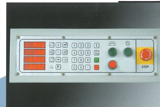
CNC Control Panel The standard fixed or optional hanging-type controls can be used for setting the saw blade up or down, tilting and cutting width dimensions. Also, there is a 30-set of program memory capacity.
