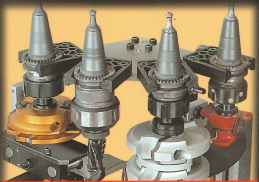
Arbeitsaggregat
