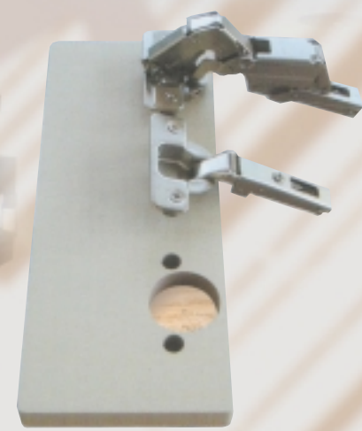
HINGE DRILLING
