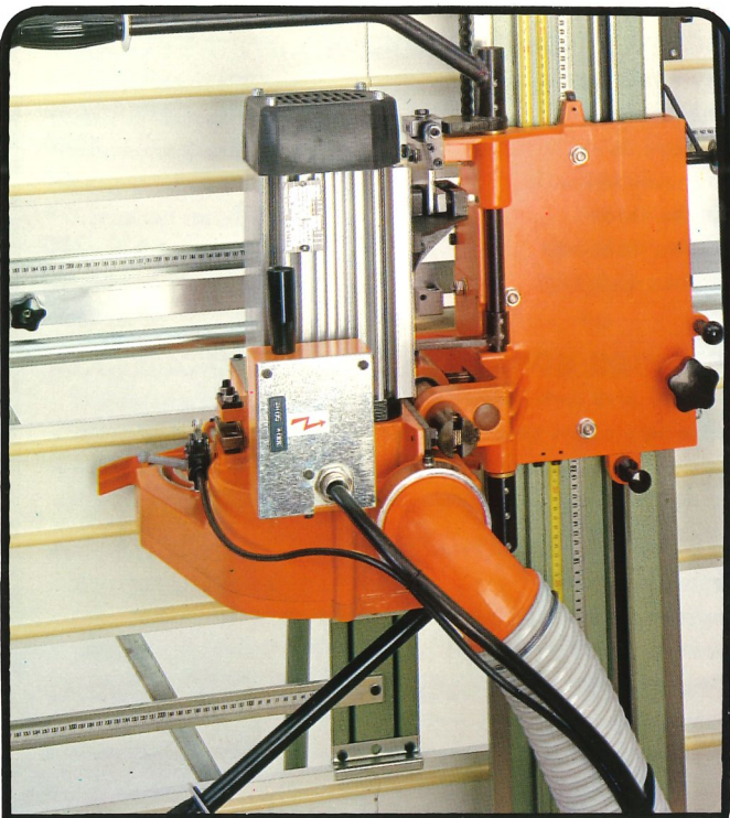
TESTA A 90° PER TAGLIO ORIZZONTALE POSITION FUER WAGRECHTEN SCHNITT ROTATION OF THE CUTTER BLOCK HEAD THROUGH 90° FOR HORIZONTAL CUTTING CABEZA PORTAHOJA A 90° PARA EL CORTE HORIZONTAL
