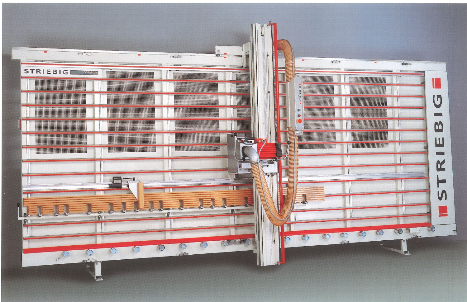
COMPACT TRK 5207
