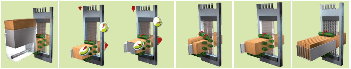
送料推臂
