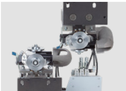
Profile scraper Unit to smooth radii or chamfers, equipped with quick change heads for fast profile change.
