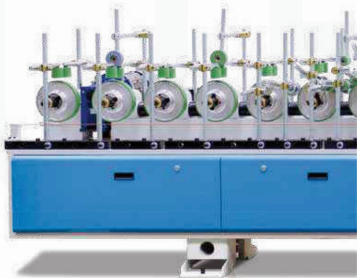
Glue grammage regulation system through PLC. (PUR)
