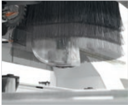
NC-controlled deflector (chip conveyor).
