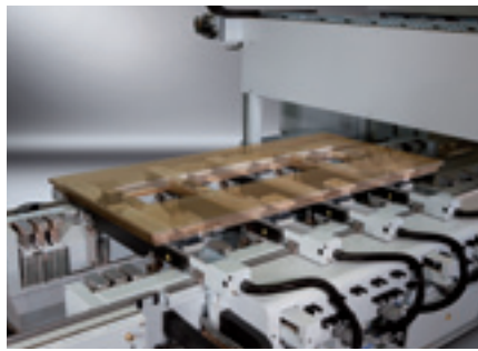
The universal clamping systems can be used simultaneously – for instance to produce front doors or semi-circular arches.
