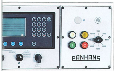
Frequency control for 8 spindle speeds. Option
