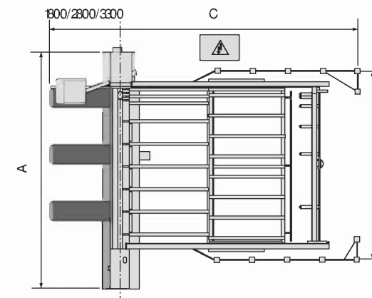
AXO500 THD
