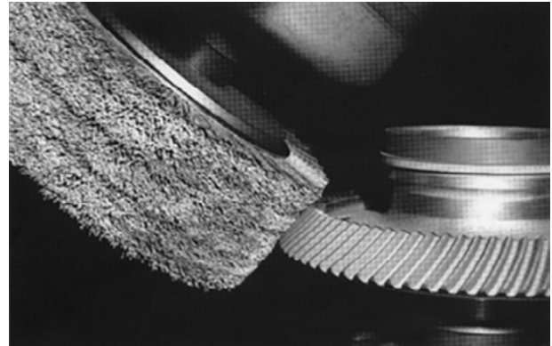
Figure 7. A Short-Trim Brush Is Used to Deburr and Finish a Gear
