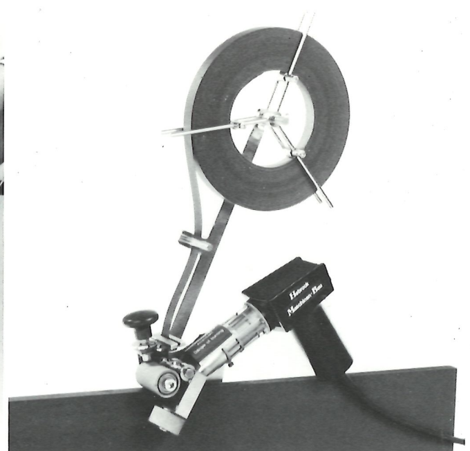
HKV 7 with powerful Leister-blast and equipment to unwind the edge material.
