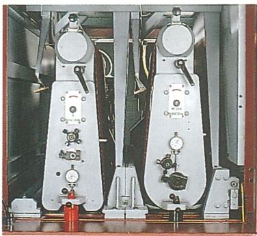
2-Aggregat Maschine
